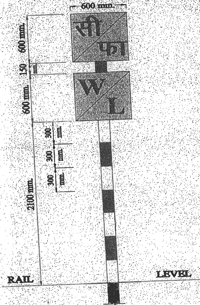
DETAILS OF WHISTLE BOARD ON THE APPROACH OF A LEVEL CROSSING
