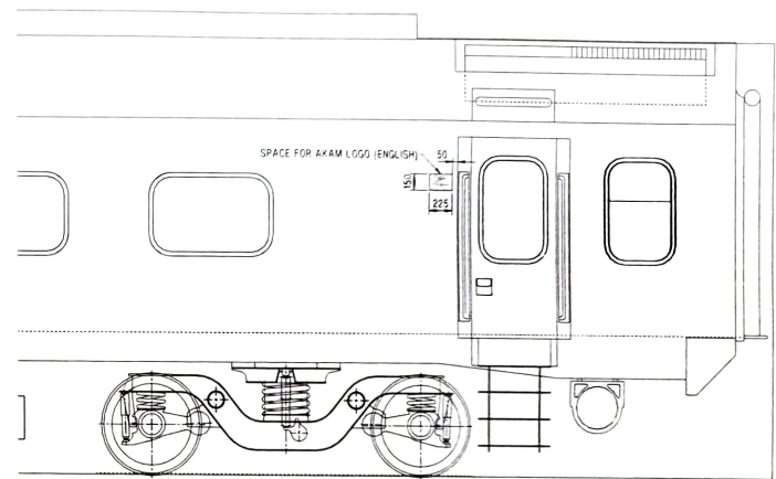
LHB TYPE COACHES
