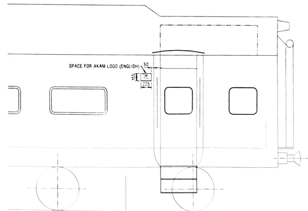
ICF TYPE COACHES
